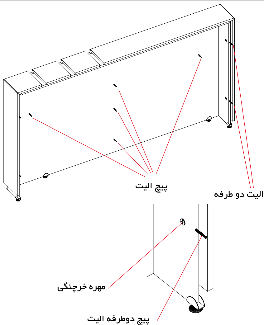
EXPLODE VIEW
