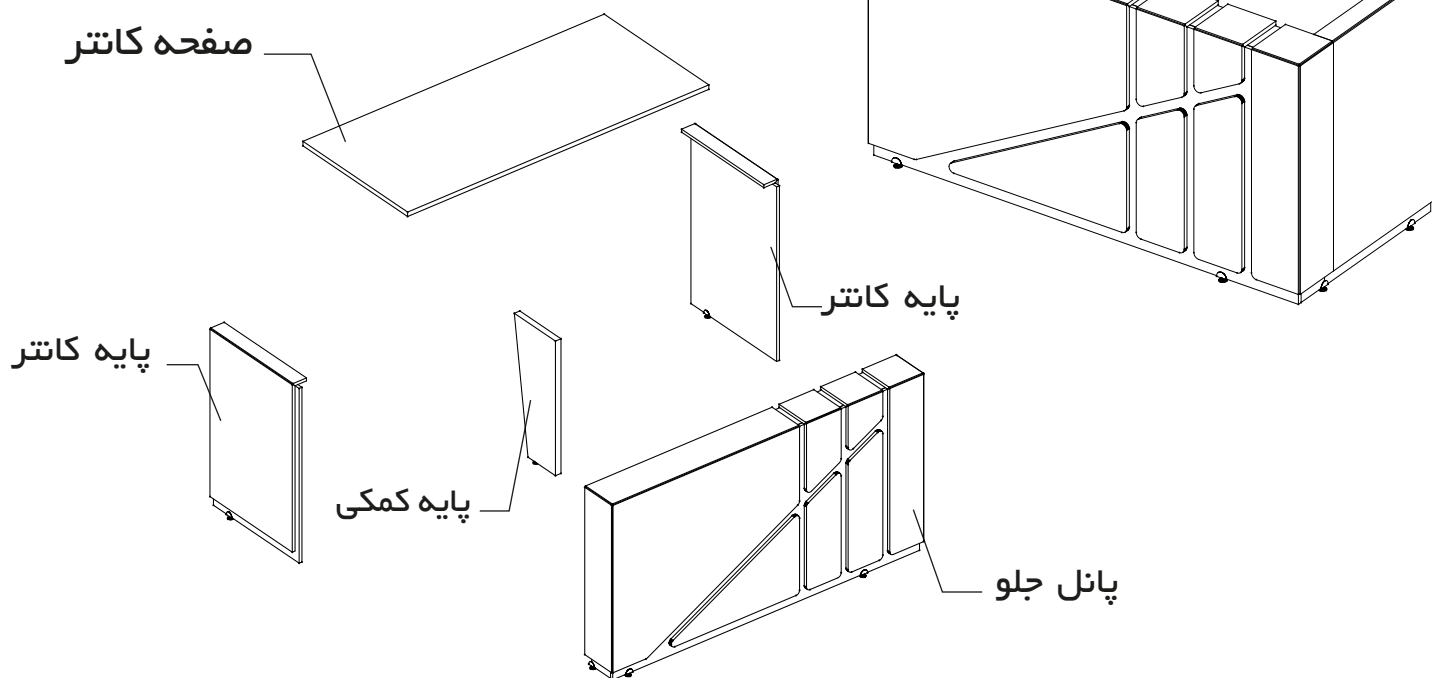
EXPLODE VIEW
